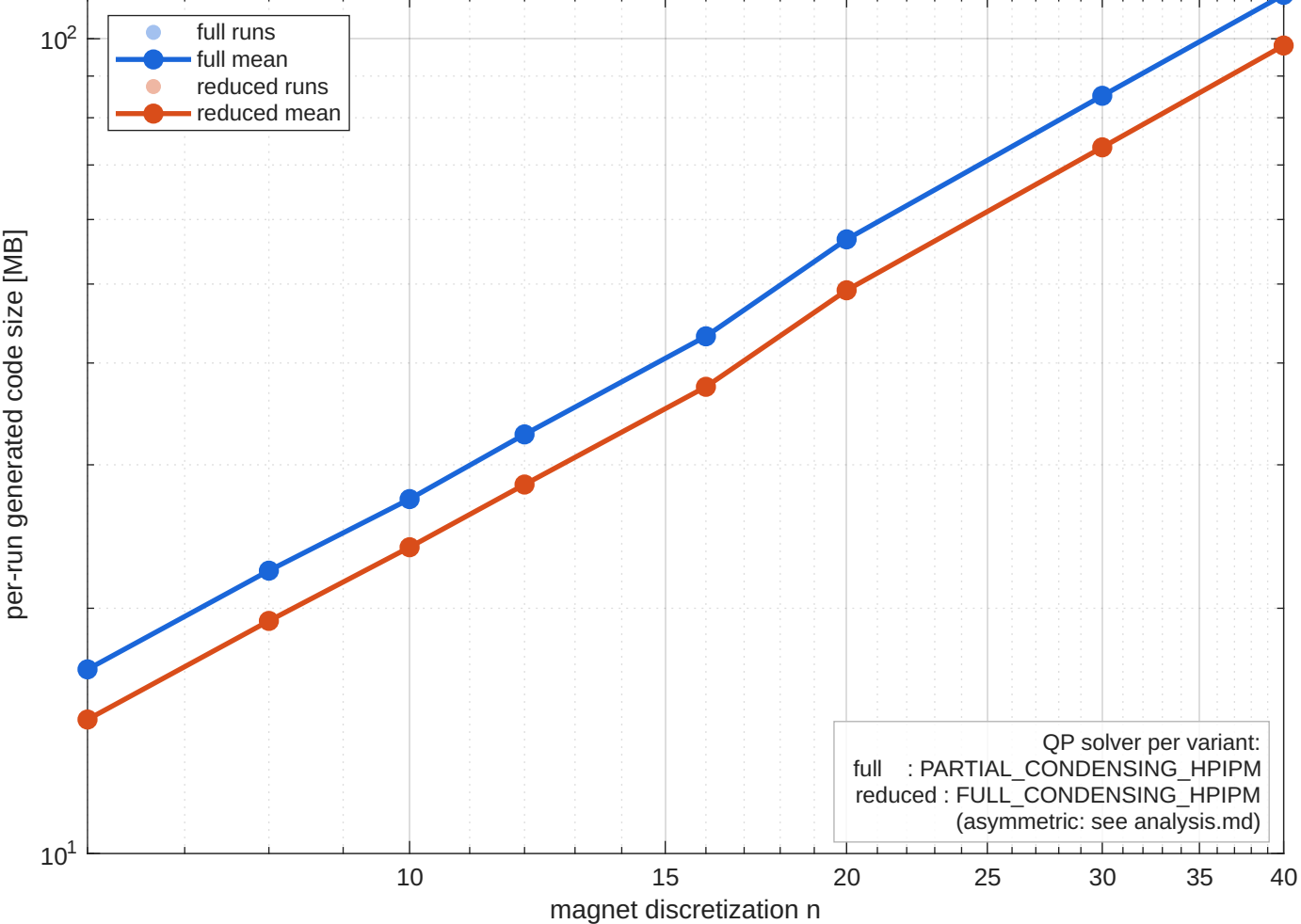
Generated C code size vs n
